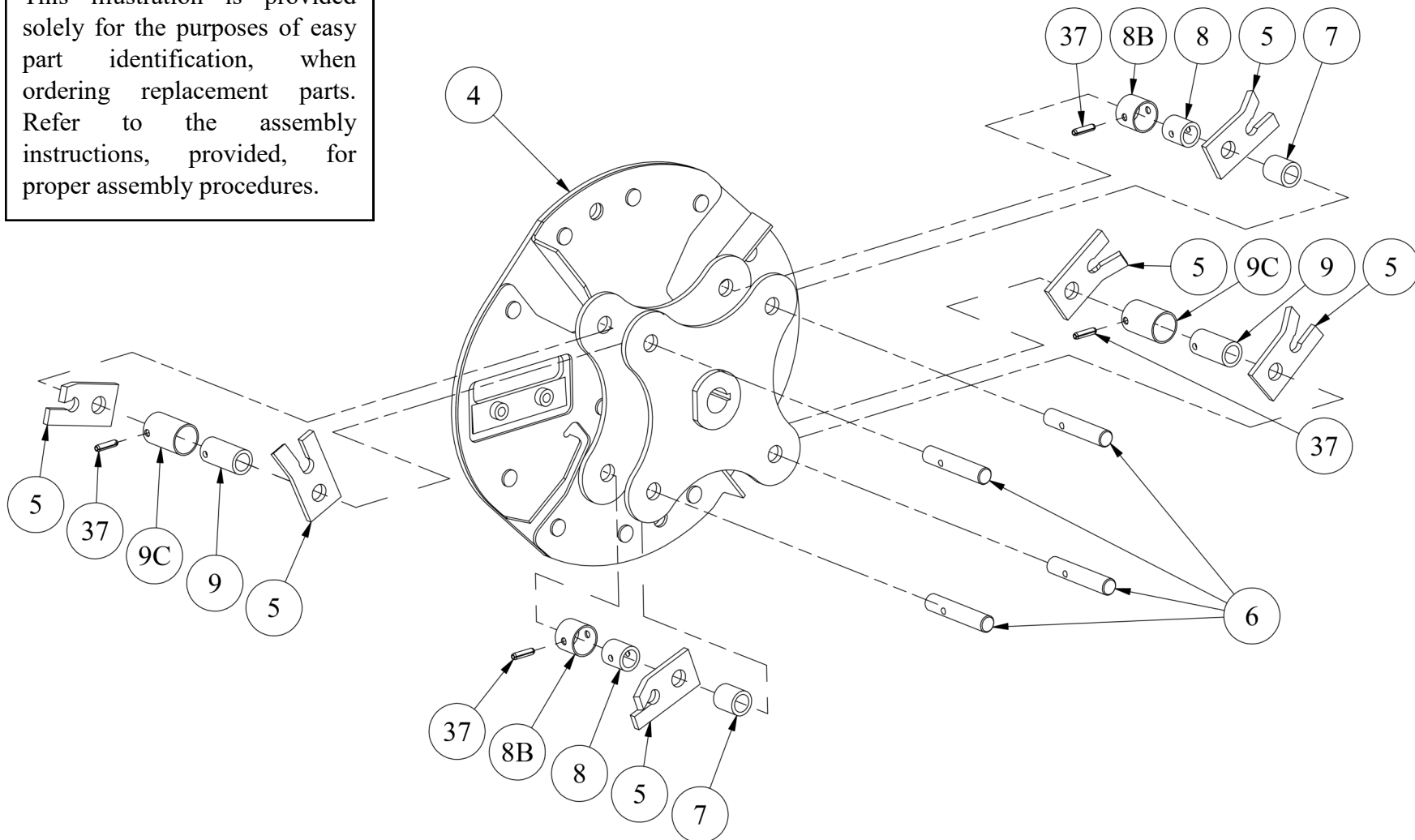
CSV-2515I Rotor Assembly Illustrated Parts-Breakdown
